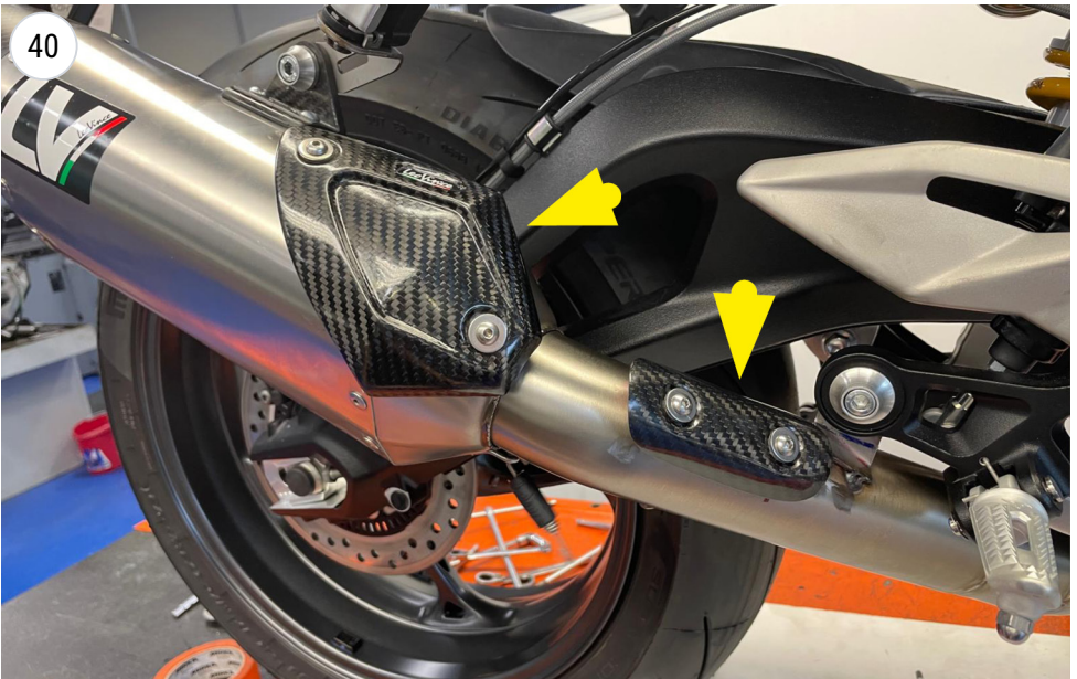
FIT THE CARBON HEAT SHIELDS
