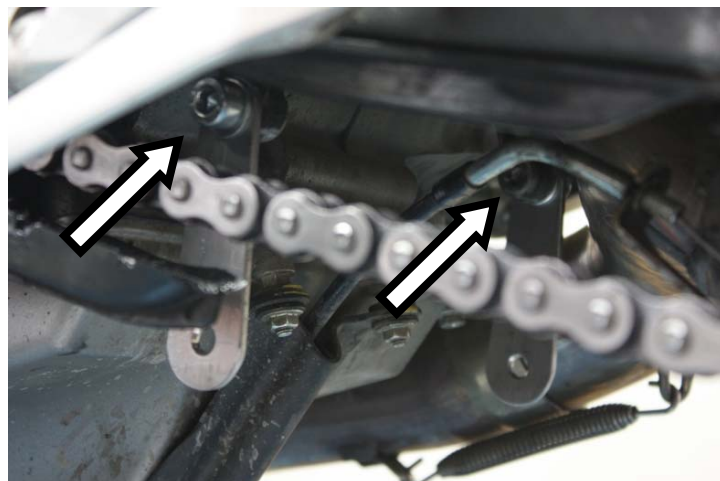
Avvitare le biellette al telaio mediante viti TCEI M8x20mm e rondelle Secure the mounting plates to the frame as shown above, using socket head cap screws M8x20mm and washers
